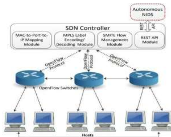
Figure 3.1: SMITE Architecture
